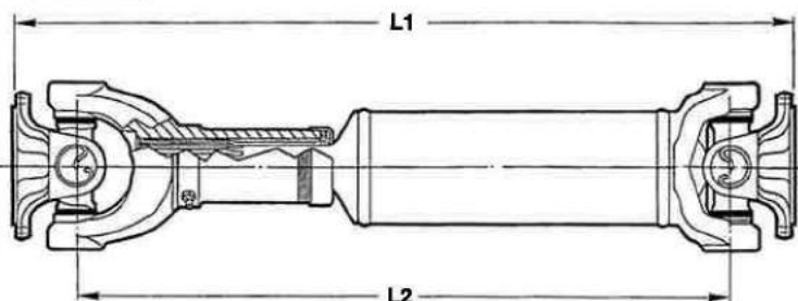
FIG 1 : TRANSMISSION LAND ROVER
